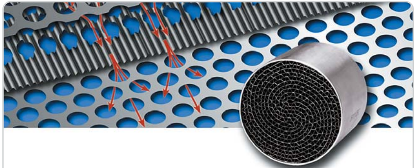
PE Foil – less weight and less backpressure
